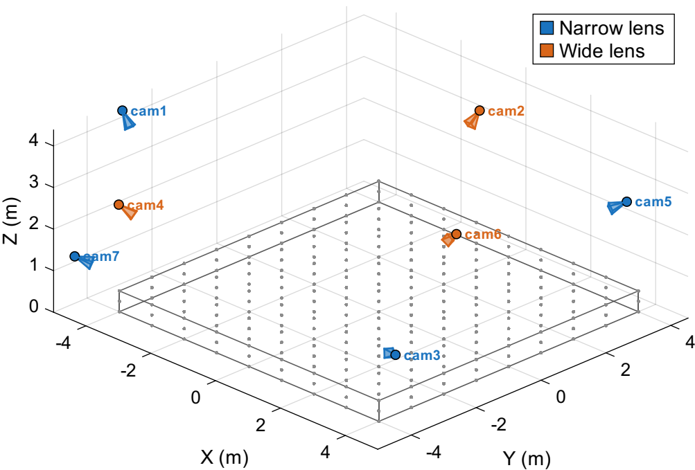
GA-best (7 cams)
